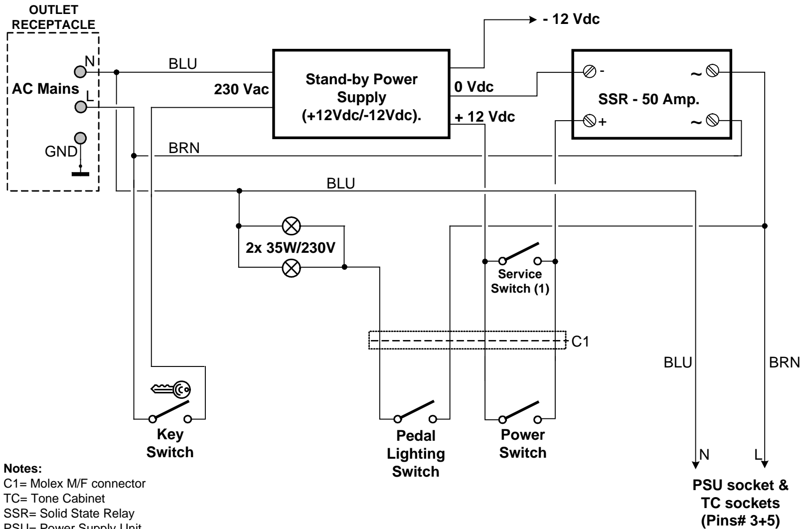
AC Mains Power Distribution
